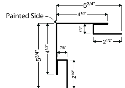
14E | TRIM FIRST OUTSIDE CORNER
