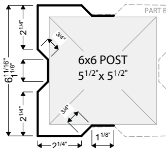
306A, 306B | 6x6 POST WRAP
