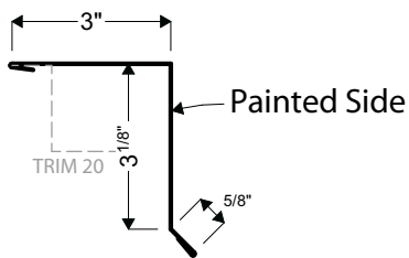
22 | ARCHITECTURAL RAKE/GABLE
