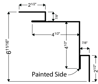
08E | TRIM FIRST INSIDE CORNER
