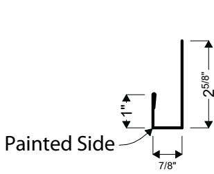
05 | J-CHANNEL
