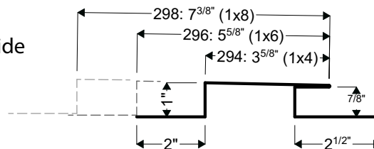
294, 296, 298 | BOARD BAND
