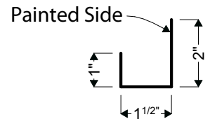
05D | REVERSE OVERSIZE J-CHANNEL
