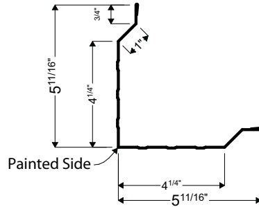
14R | OUTSIDE CORNER (RIBBED)
