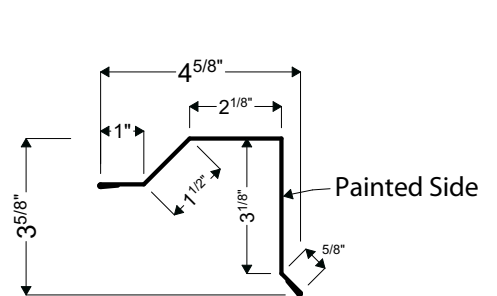
06E | STANDING SEAM GABLE
