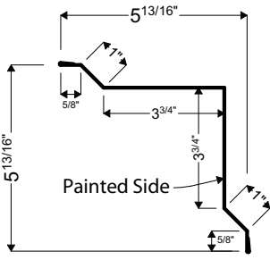
08 | INSIDE CORNER
