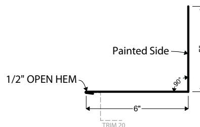
50C | STANDING SEAM SIDEWALL
