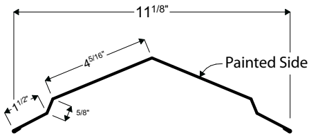
01 | RIDGE CAP
