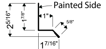
13 | L BASE TRIM
