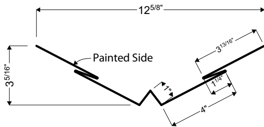
02C | CLEATED VALLEY
