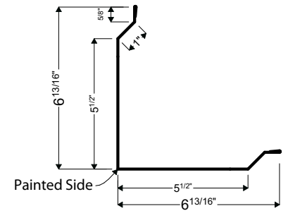
14B | OVERSIZE OUTSIDE CORNER
