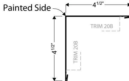
14D | ARCHITECTURAL CORNER
