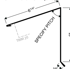
31C | JUMBO ARCH'L PEAK FLASHING
