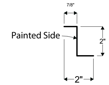
20D | Z TRIM D (STANDING SEAM)
