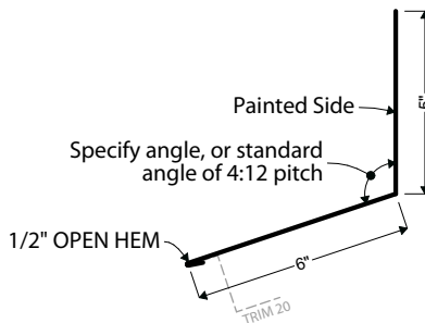
50B | STANDING SEAM ENDWALL
