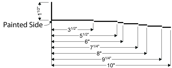
103B, 105B, 106B, 107B, 108B, 109B, 110B | POST TRIM B
