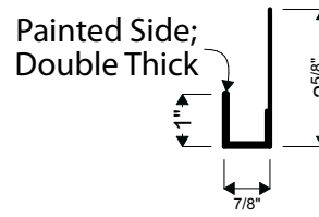
05C | FULL WRAP J-CHANNEL
