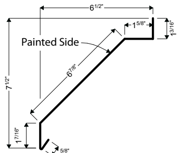
24 | TRACK COVER
