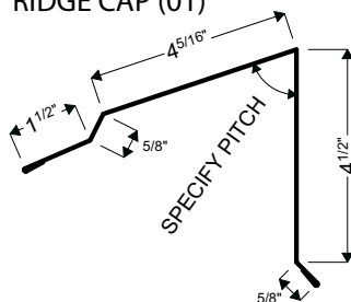
31 | PEAK FLASHING
