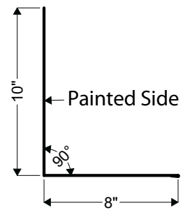
04F | JUMBO SIDEWALL
