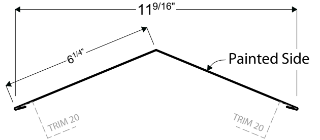
01B | RIDGE CAP - ARCHITECTURAL
