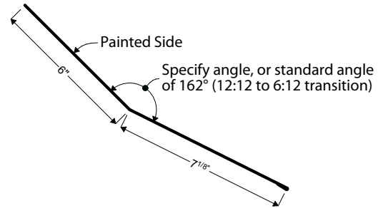
04 | PITCH BREAK (TRANSITION)
