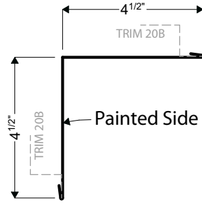
08B | ARCHITECTURAL INSIDE CORNER
