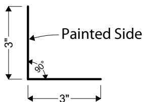
25 | UNIVERSAL FLASHING
