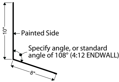
04D | JUMBO ENDWALL
