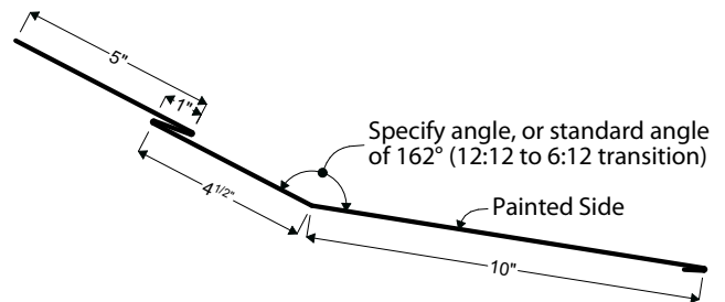
04G | CLEATED PITCH BREAK
