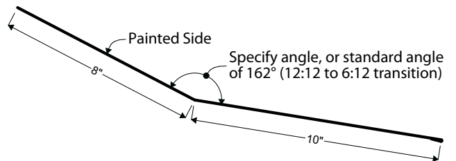
04B | JUMBO PITCH BREAK (TRANSITION)
