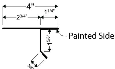
07B | STANDING SEAM EAVE
