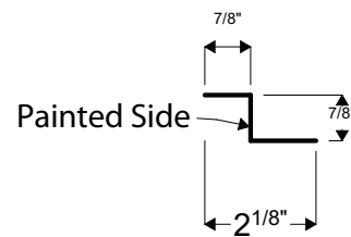
20B | Z TRIM B (TUFF-RIB; BOARD & BATTEN)
