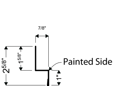
15 | WALL LITE FLASHING
