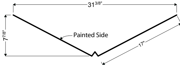
02B | JUMBO VALLEY
