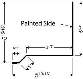
18 | ROOF TO WALL FLASHING
