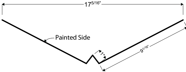
02 | VALLEY
