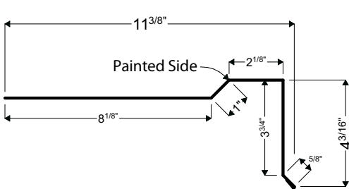
03 | PROW FLASHING
