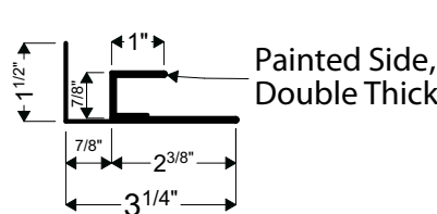
16C | FULL WRAP FJTRIM
