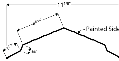
01R | RIDGE CAP - RIBBED
