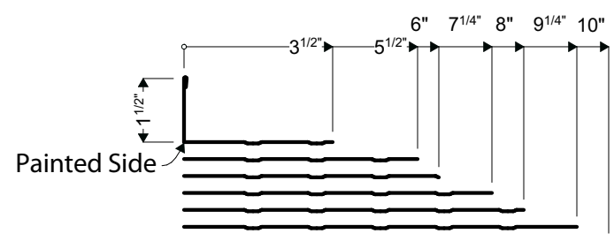
103R, 105R, 106R, 107R, 108R, 109R, 110R | RIBBED FASCIA
