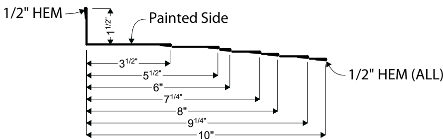
103D, 105D, 106D, 107D, 108D, 109D, 110D | INSIDE ANGLE
