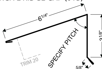
31B | ARCHITECTURAL PEAK FLASHING
