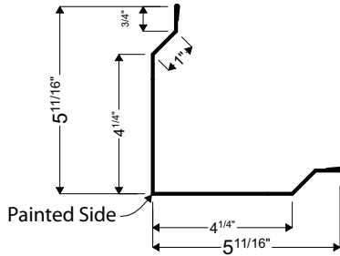
14 | OUTSIDE CORNER
