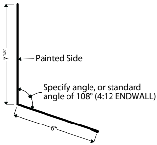
04C | ENDWALL
