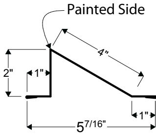
12 | SNOW GUARD
