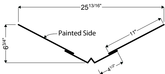
02D | JUMBO CLEATED VALLEY
