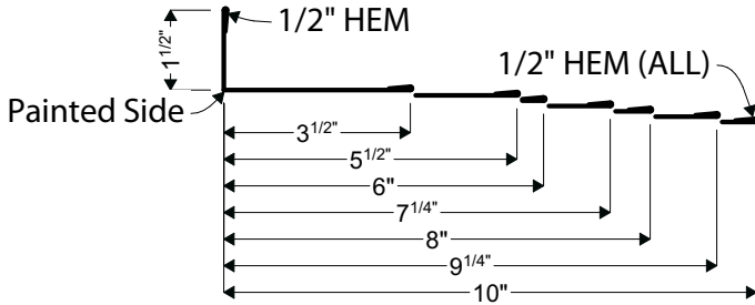
103, 105, 106, 107, 108, 109, 110 | POST TRIM
